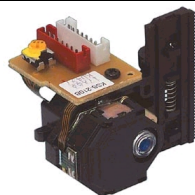
KSS 210 B
